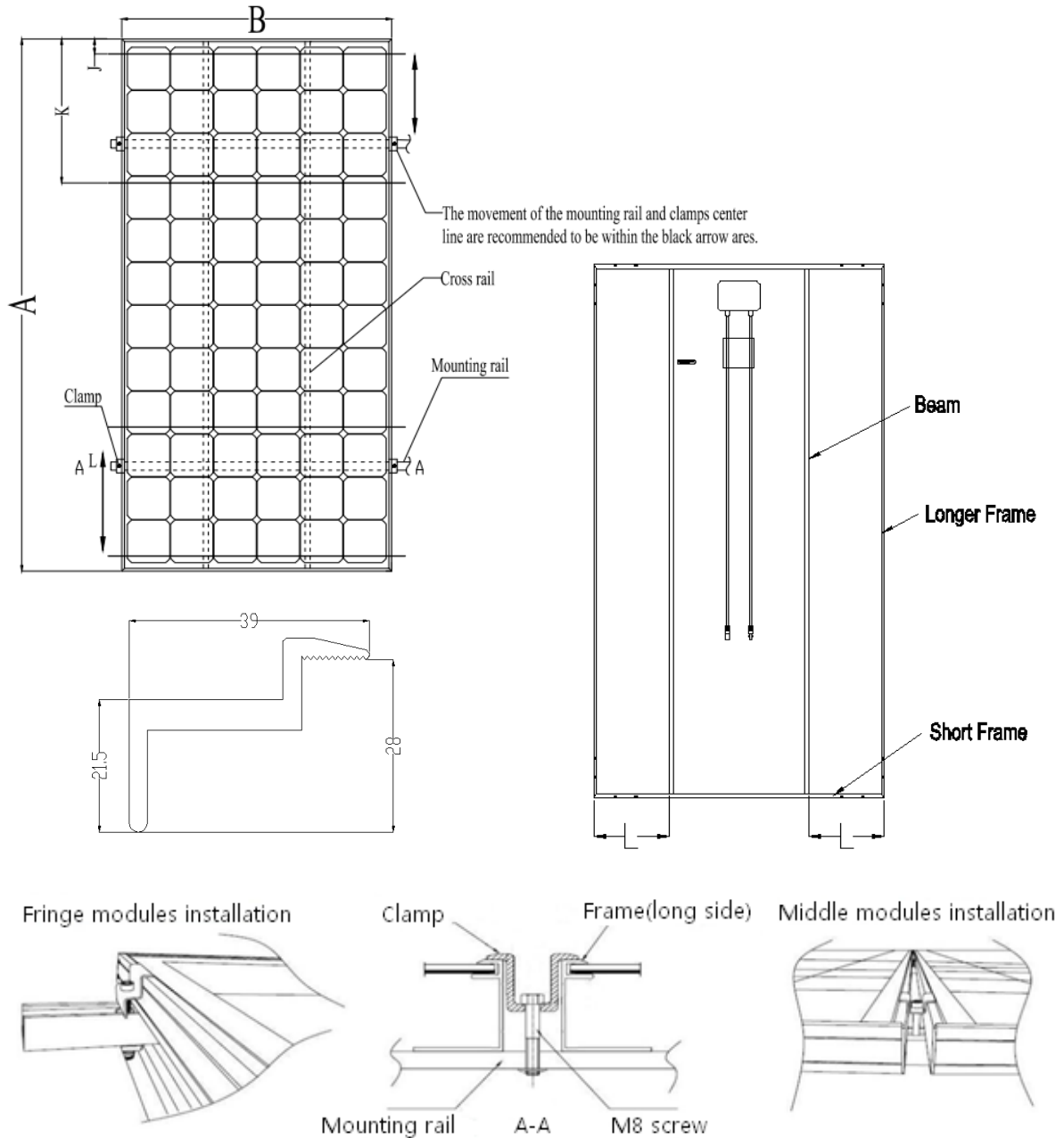
Figure 4: Light PV module installed at long side with Clamp fitting method
