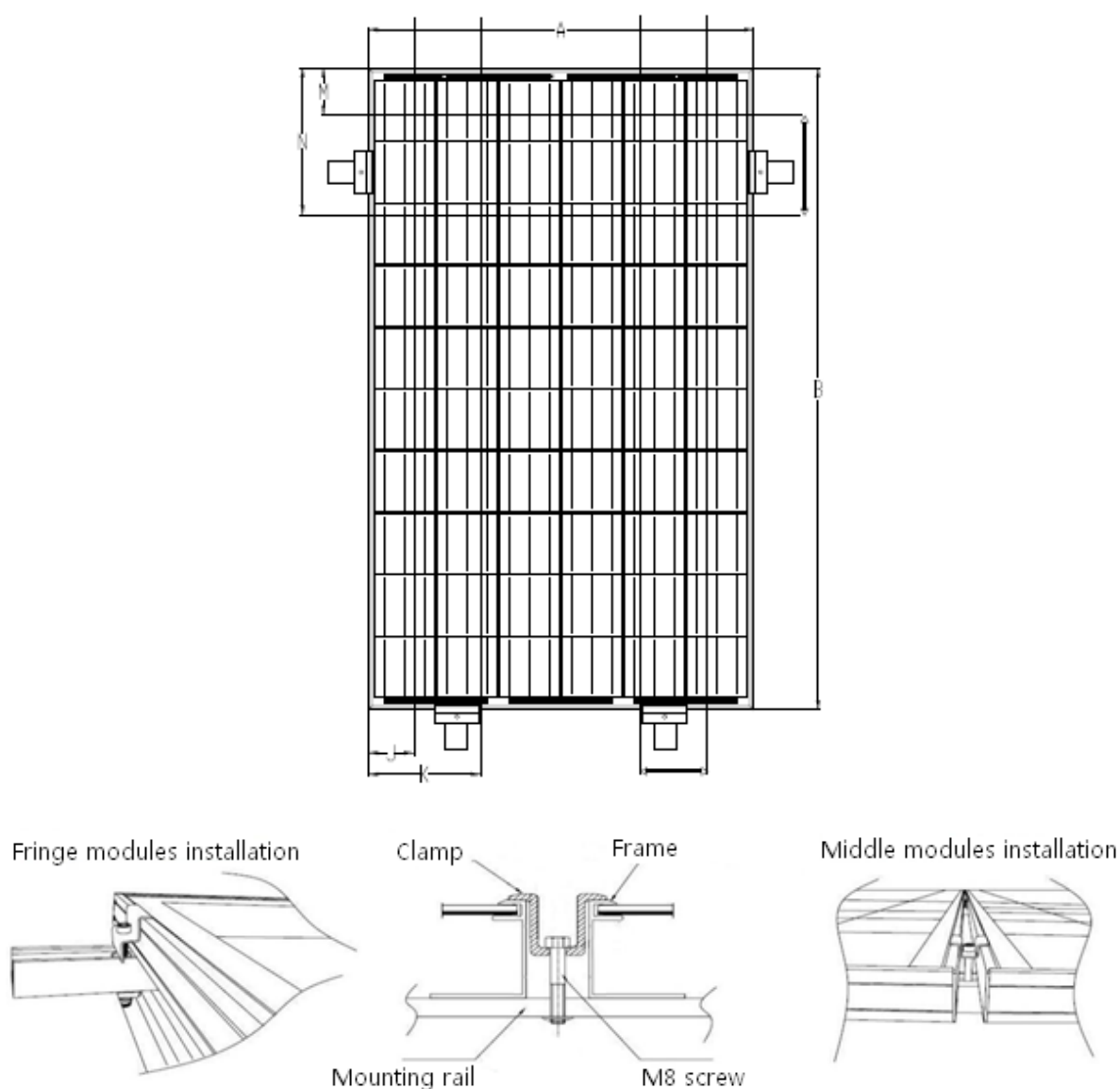
Figure 6: PV module installed at long and short side with Clamp fitting method
