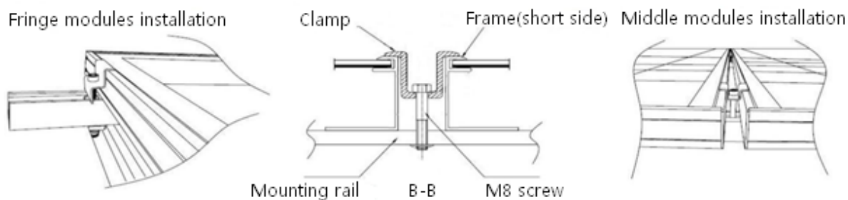
Figure 5: PV module installed at short side with Clamp fitting method
