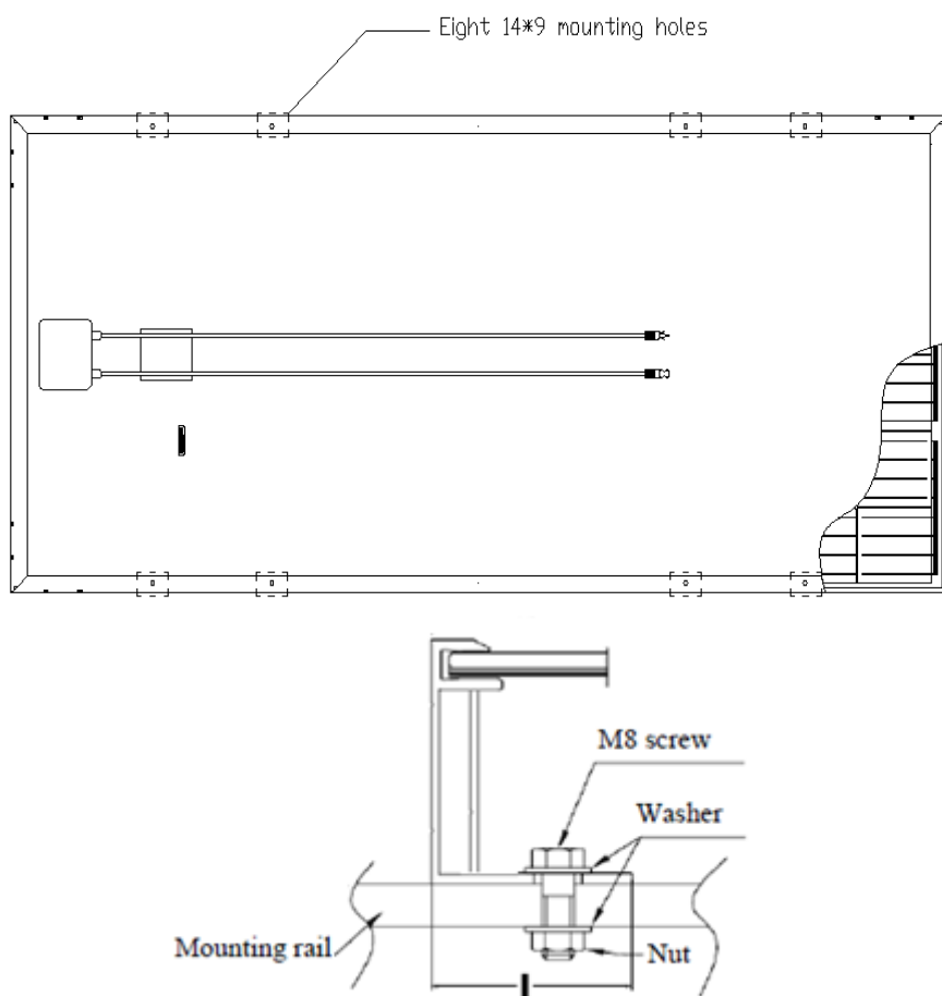
Figure 2: PV module installed with Screw fitting method
