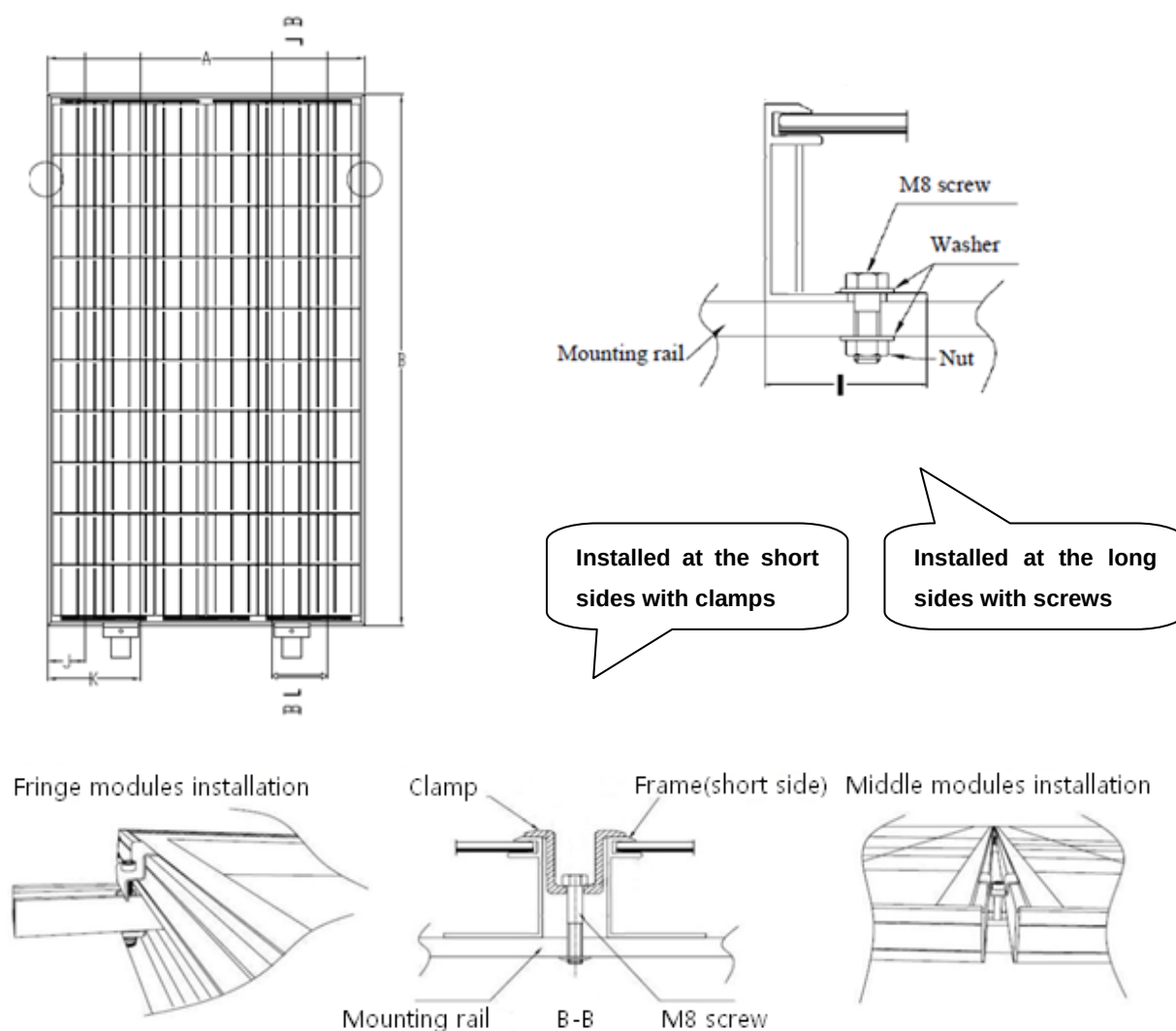
Figure 7: PV module installed at long and short side with Screws and Clamps respectively
